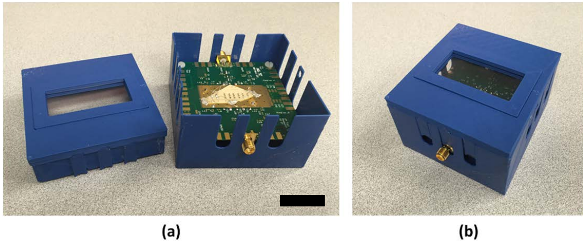
Figure 4.10. (a) The lid and the base made of ABS plastic using a 3D printer. The scale bar is 1 inch. (b) Closed housing box with SMA connections.
