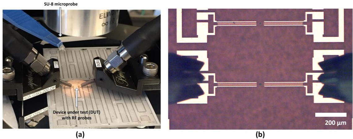
Figure 5.2. (a) Testing of devices from the third photomask set. (b) Microscope image showing probing of large aperture SAW devices from the first photomask set with GSG type RF probes.
