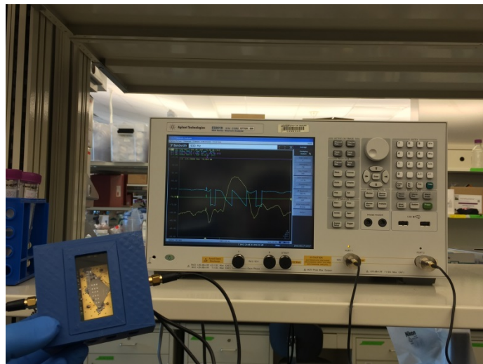
Figure 5.26. Integrated system showing the VNA, PCB, and the measured SAW device in the 3D printed housing.
